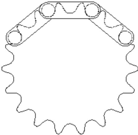
Standard Rollers Double Duty
