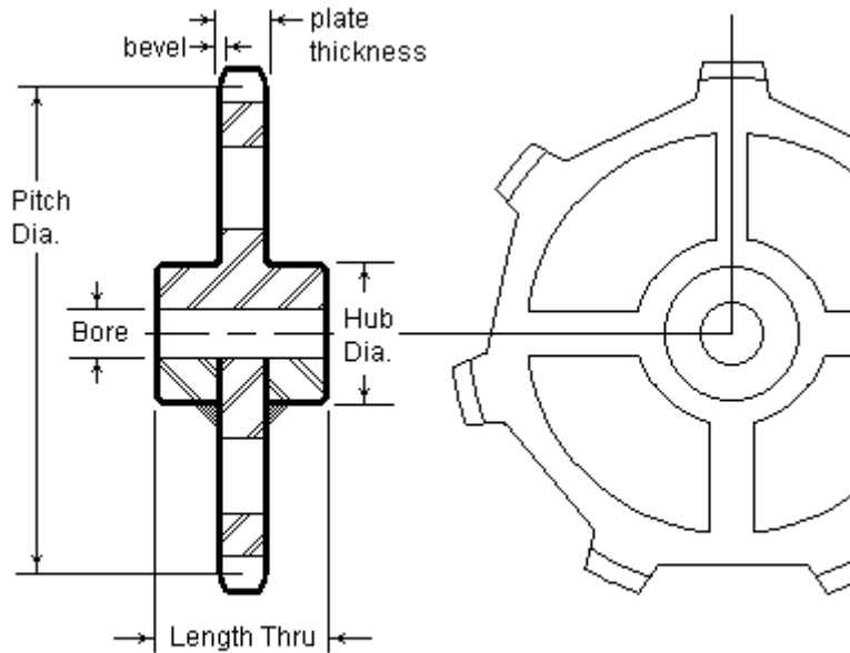
458 and 678 series - all spoke wheel design
