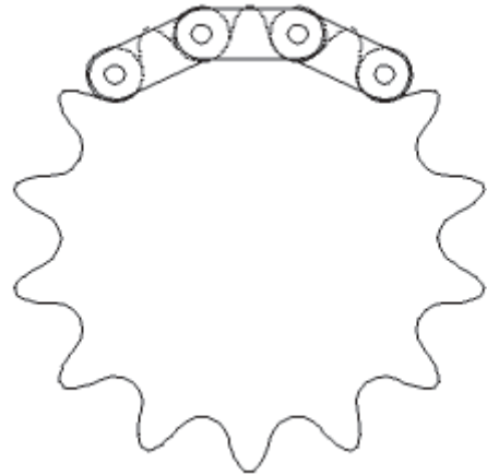
Oversize Rollers Single Duty
